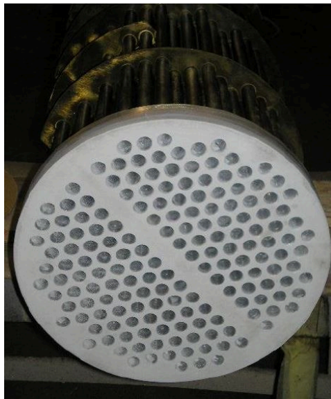
Example of a tube bundle cleaned and refurbished along with water box.
